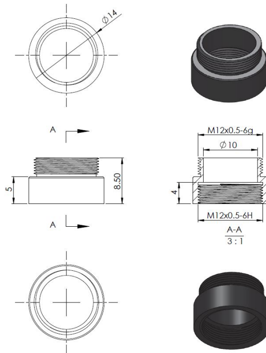
M12 extension ring 5 mm, anodized
