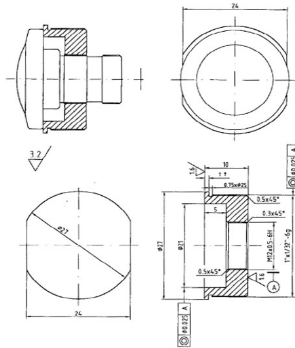
OEM Adapter s-mount-c-mount - high version
